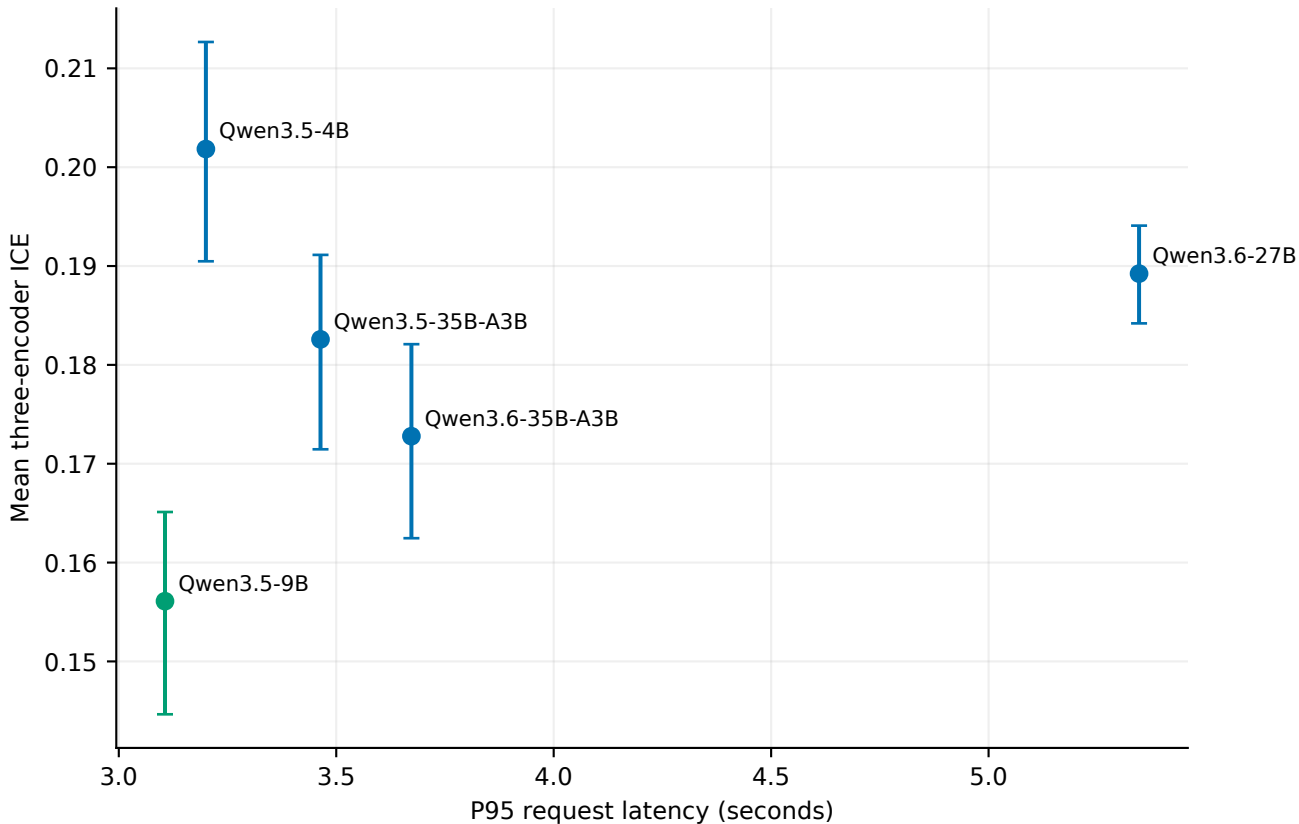
Descriptive quality-latency view Direct comparisons only within identical concurrency/TP groups
