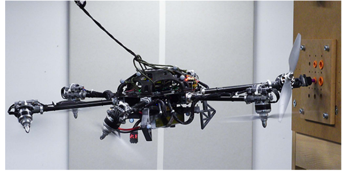
Fig. 1. Omnidirectional tilt-rotor aerial robot screwing a bolt into a wall. The robot can smoothly transition its arms from flying mode (propellers on) to interaction (propellers off) with our novel allocation method. Video: https://youtu.be/ybT80MyB9_Y .
