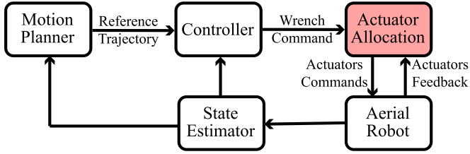
Fig. 3. General control architecture for tilt-rotor aerial robots. The pose controller compares the current odometry to a reference trajectory and produces a wrench command. The wrench command is finally allocated to the actuators of the robot, namely servomotors and propellers, to generate the desired wrench which drives the platform. In this work we focus on the allocation block, highlighted in red.
