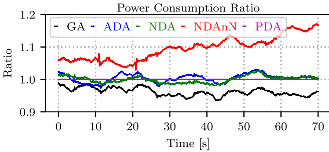
Fig. 10. Power usage ratio between PDA and the other allocation methods during the slow Figure-8 trajectory. GA is up to 6% more efficient than the other differential methods, which have similar consumptions. NDAAnN increases the average propeller speeds over time, leading to a power consumption up to 18% higher than the PDA method. The power consumption is computed using (15) with J = 4.5e^{-4} \text{ Kg m}^2 and d = 3.5e^{-7} \text{ N m s}^2 . The servomotors power consumption is two orders of magnitude smaller and thus negligible.
