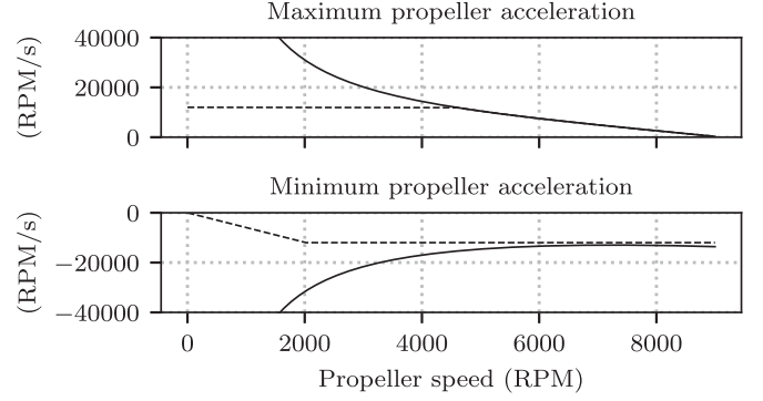
Fig. 5. Example acceleration limit curves (solid lines) from the propellers power balance in (15). The dashed lines represent the saturated versions of the curves, where the maximum and minimum accelerations have been capped to represent the internal software ESC limits. For very low propeller speeds, the drag torque has a very low effect, leading to very high acceleration and deceleration limits. As speed increases, the quadratic drag force overtakes the electrical torque, leading to a reduction in the maximum acceleration and deceleration, until the acceleration becomes zero when the propeller reaches the maximum speed. The curves were obtained with \eta = 0.8 , V = 23V , \bar{I} = -\underline{I} = 17A , J = 4.5e^{-4} Kg m^2 , d = 3.5e^{-7} N m s^2 and \bar{\omega} = -\underline{\omega} = 1.3e^4 RPM/s .
