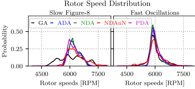
Fig. 9. Comparison of rotor speeds distributions between the different allocation methods. When the secondary objective is not present (Normalized Differential Allocation with no Nullspace objectives (NDAAnN)) or in case of the GA, the rotor speeds distribution is wider and the propellers are pushed closer to their limits.
