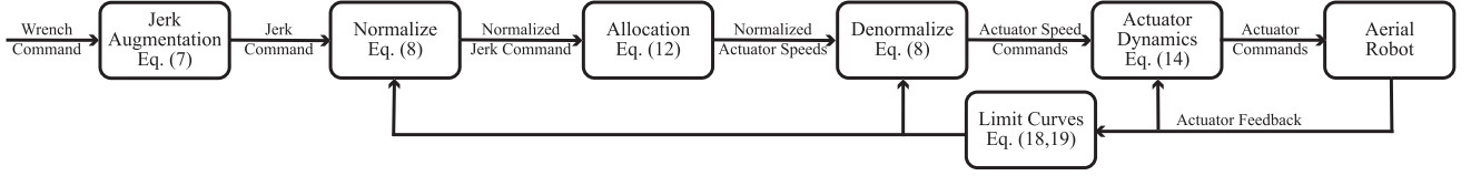
Fig. 4. Proposed DA scheme. We first augment the wrench command to generate a jerk command, we then normalize it and allocate into numerically stable normalized joint speeds. Finally, we invert the actuator dynamics to obtain the desired tilt angles and propeller speeds to command the Aerial Robot.
