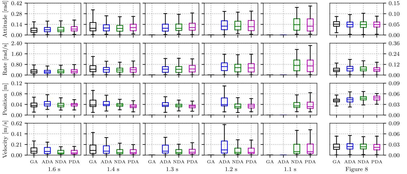
Fig. 14. Tracking results from the different allocation methods. Top to bottom rows: attitude, angular velocity, position and linear velocity errors. Left to right columns: increasingly fast sinusoidal trajectories, from a period of 1.6 s to 1.1 s, ending with a slow Fig. 8 trajectory. If no data is present, the corresponding allocation diverged while following the trajectory.
