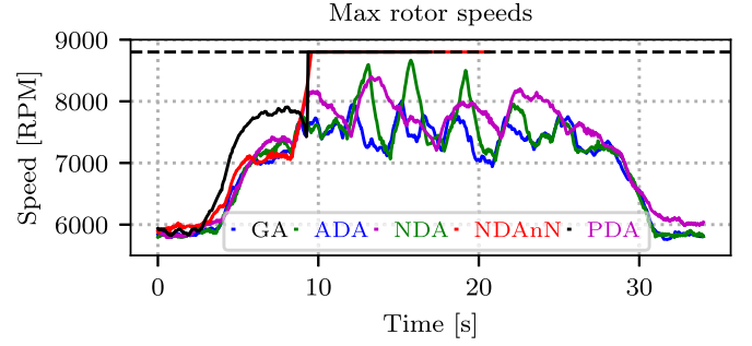
Fig. 11. Maximum rotor speeds experienced during the cartwheel trajectory by the different methods. The speed limit allowed by the ESCs is 8800 RPM (dashed line). GA and NDAAnN both hit the saturation and diverge, while the other methods keep the propellers away from the limit.
