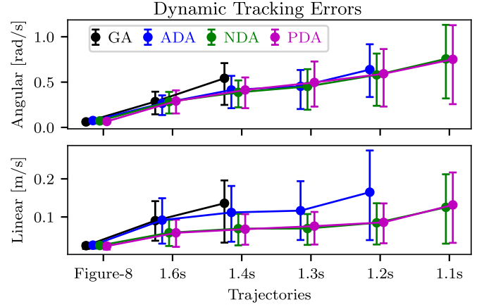
Fig. 8. Mean and quartiles of the linear and angular tracking velocity errors achieved by the geometric (Geometric Allocation (GA)) and differential (Augmented Differential Allocation (ADA), Normalized Differential Allocation (NDA), Power Differential Allocation (PDA)) allocations. When data from an allocation is missing for a specific trajectory, it means that the method failed to complete the trajectory. The use of actuator dynamics allows PDA and NDA to complete all trajectories.
