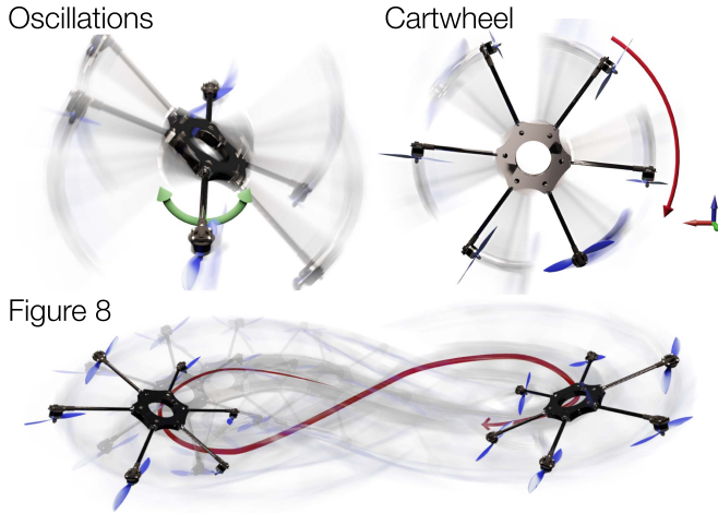
Fig. 7. Illustration of evaluation trajectories. Top Left: Sinusoidal motion around body axes with increasingly faster cycle times, the roll motion is visualized. Top Right: Cartwheel trajectory, in which the robot is commanded to fly upright in the vertical plane and rotate slowly around the perpendicular axis. Bottom: Fig. 8 that smoothly excites all axes – similar to the well-known ‘Lazy 8’ in aviation.
