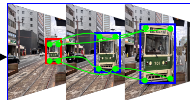
Tracked BBox
