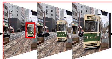
Predicted BBox
