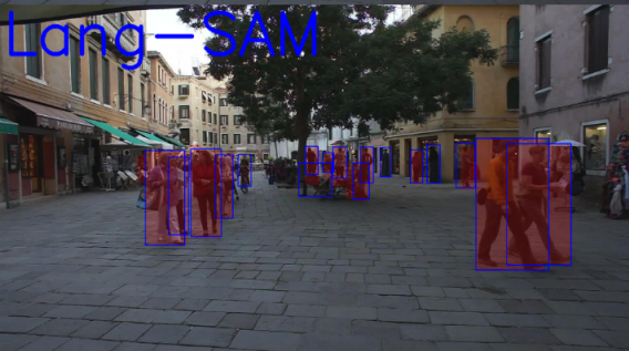
Proposed Method
