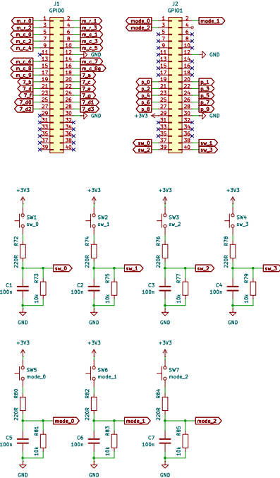
Figure 3-20 GPIO Pin Arrangement
