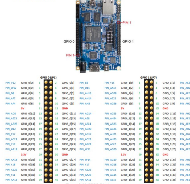
Figure 3-20 GPIO Pin Arrangement
