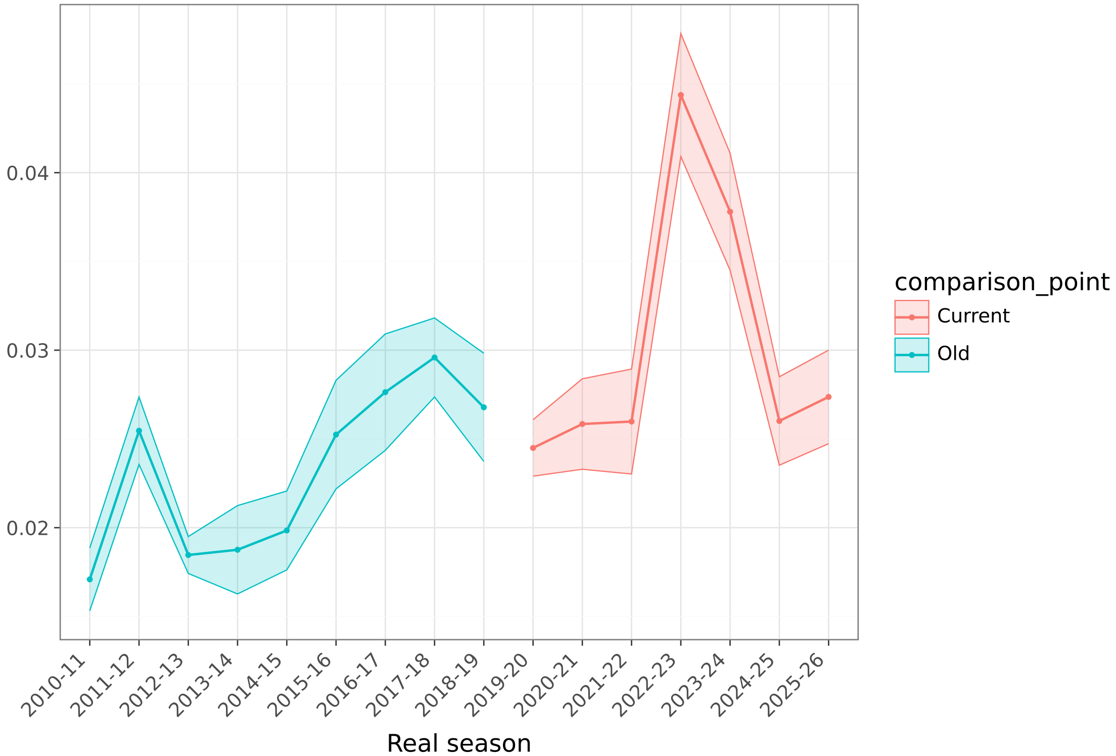
Wasserstein distance
