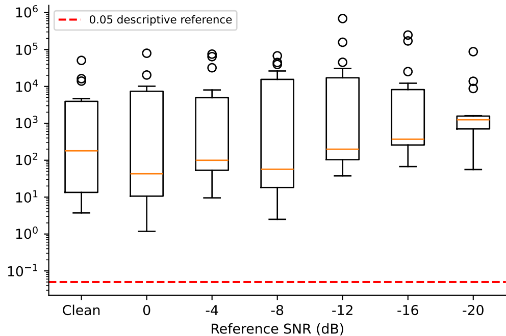
AlexNet
