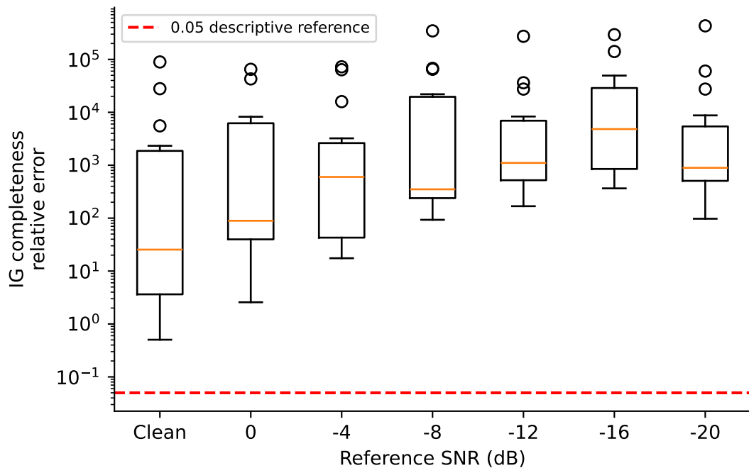
CNN+Transformer
