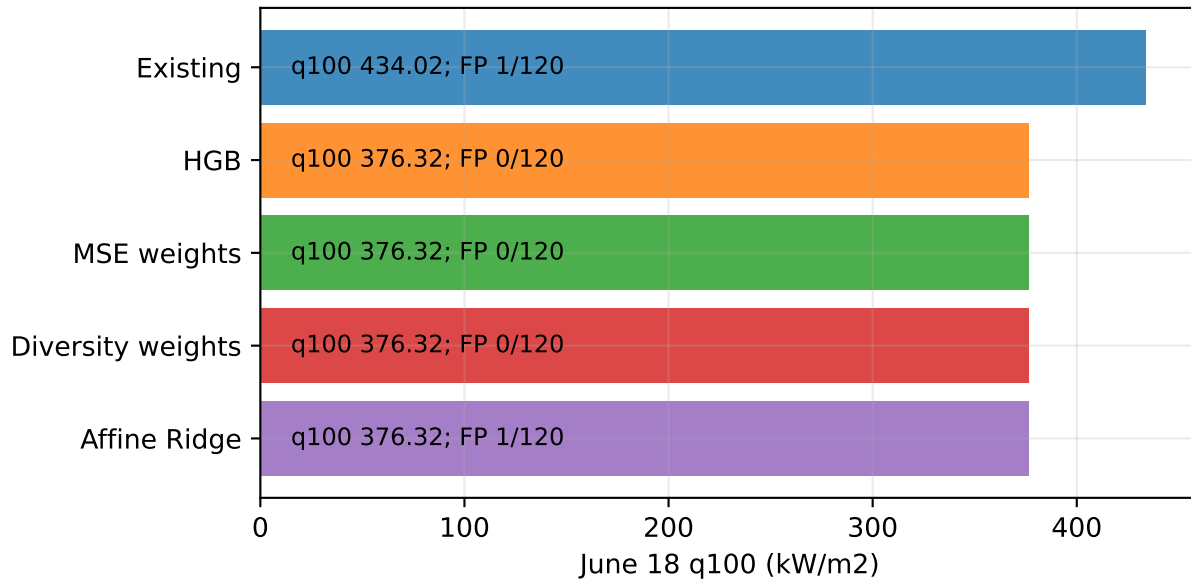
Clean q100 and pre-ONB false alarms
