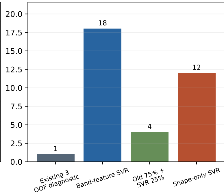
False positives / 675
