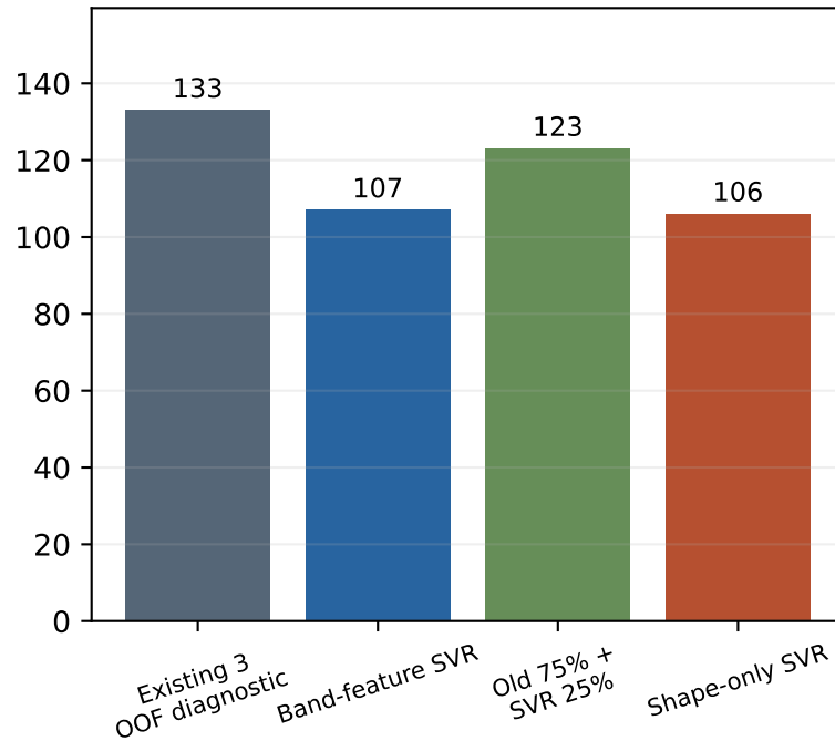
False negatives / 945
