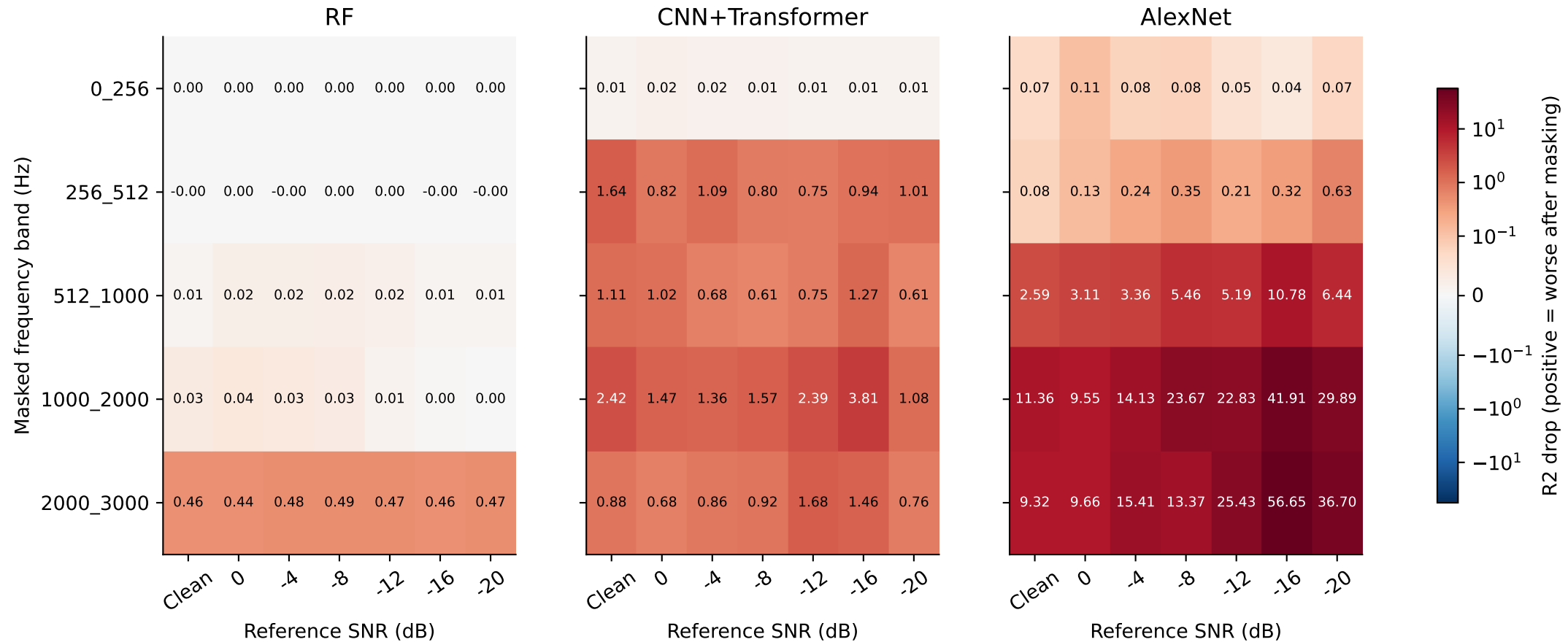
Mean fold-local WAV R2 drop after masking; unequal band widths; shared symmetric-log color scale
