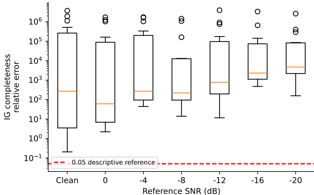
CNN+Transformer
