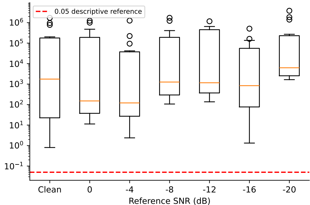
AlexNet
