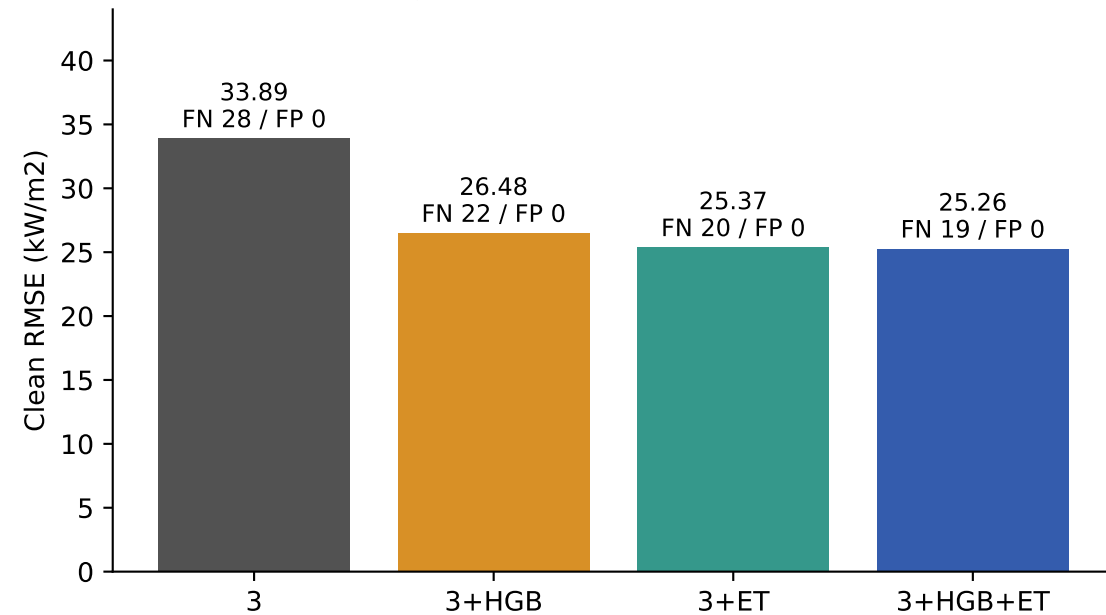
Seed 44: original models and their ratios retained
