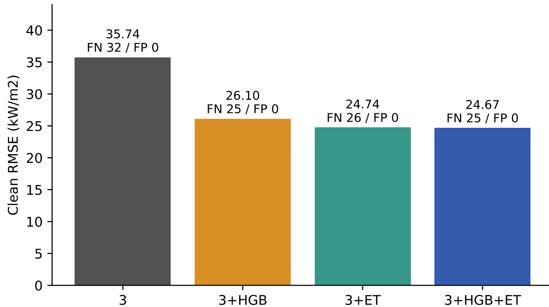
Seed 43: original models and their ratios retained
