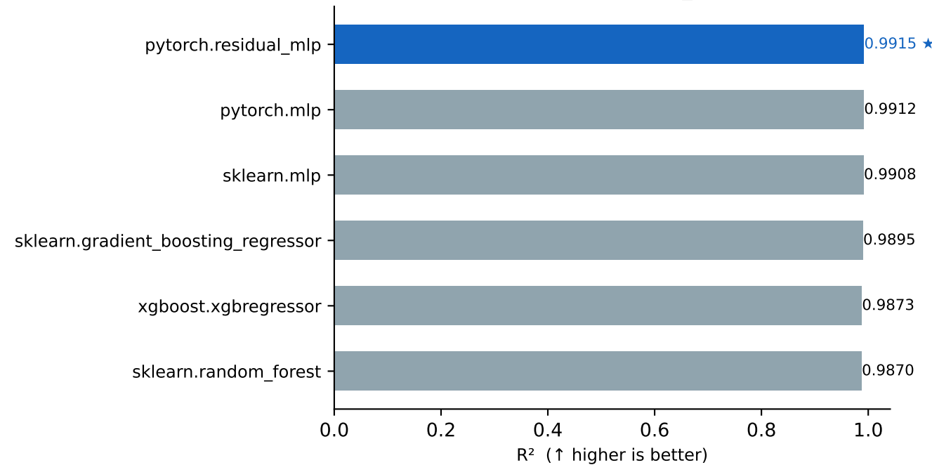
synthetic.regression_1d — R 2
