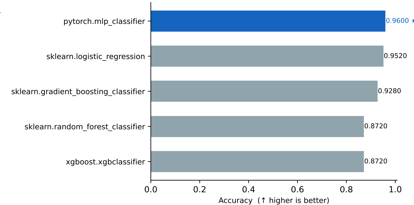
synthetic.classification_binary — Accuracy
