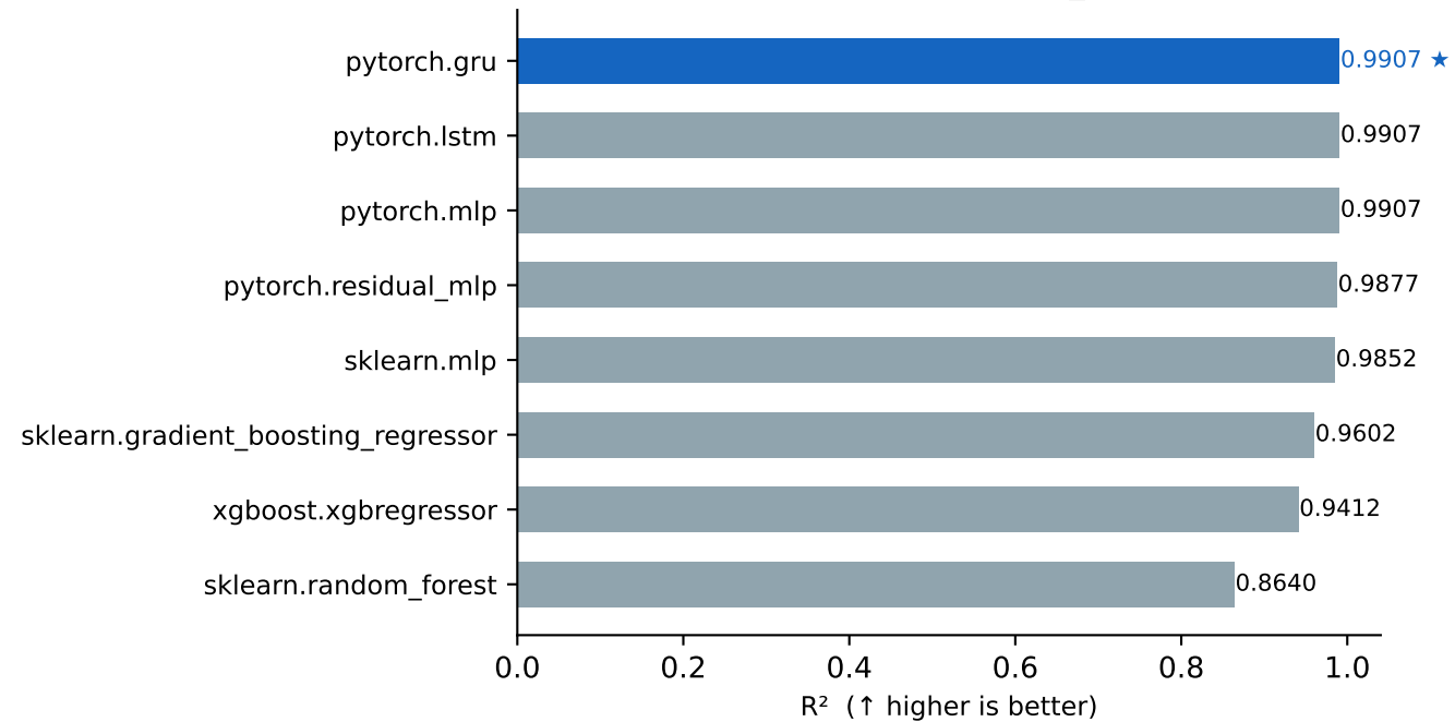
synthetic.multioutput_2d — R 2
