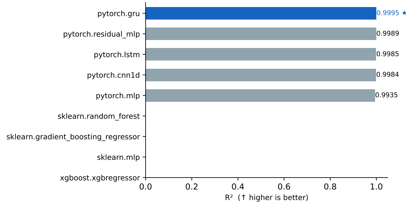
synthetic.regression_1d — R 2
