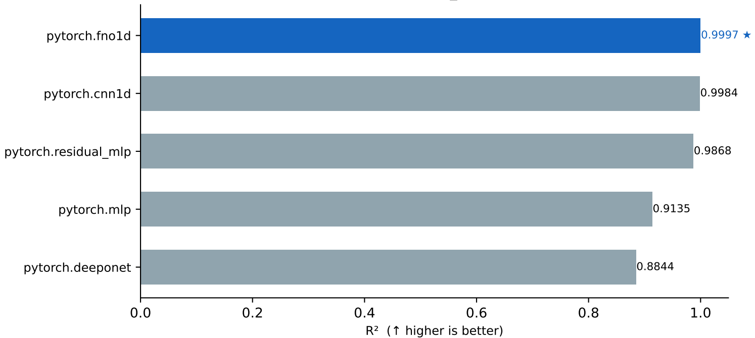
pde.burgers_1d — R 2
