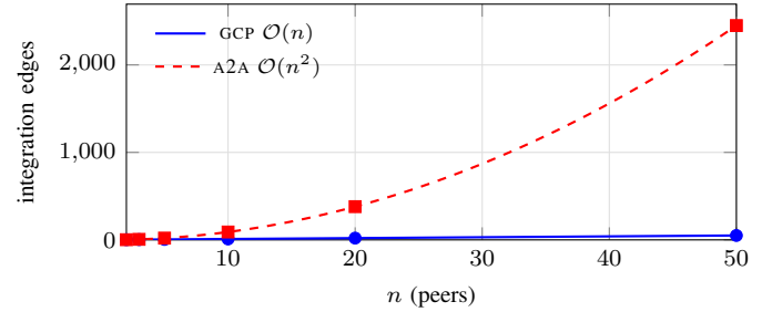
Fig. 2. Integration edges vs. peer count n . Curves are the closed-form C_{GCP}(n) = n and C_{A2A}(n) = n(n-1) ; markers are the Table II values.
