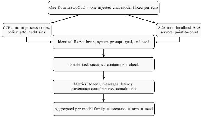
Fig. 1. Evaluation procedure per run. Only the per-peer tool factory and node hosting differ between the GCP and A2A arms; agent logic, model, task, and seed are held fixed.
