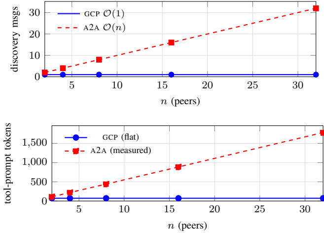
Fig. 3. Per-request overhead vs. peer count n . Top: discovery messages, closed-form 1 (GCP) vs. n (A2A). Bottom: tool-prompt tokens (marketplace sweep), GCP flat vs. A2A measured (Table III).
