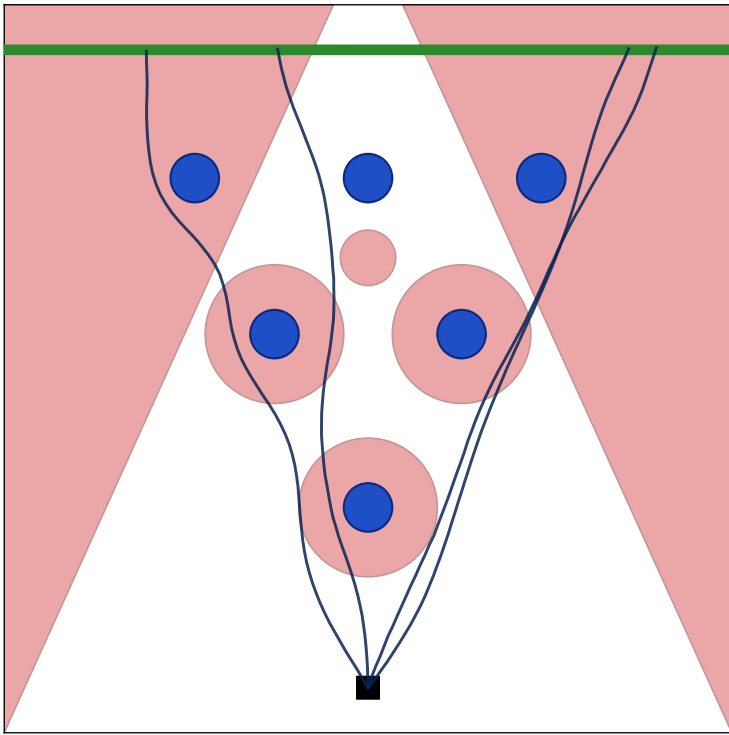
No guidance
