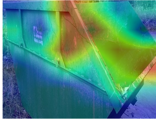
Grad-CAM: needs_collection (1.00)
