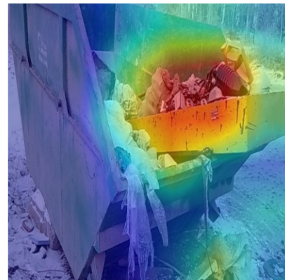
Grad-CAM: needs_collection (1.00)
