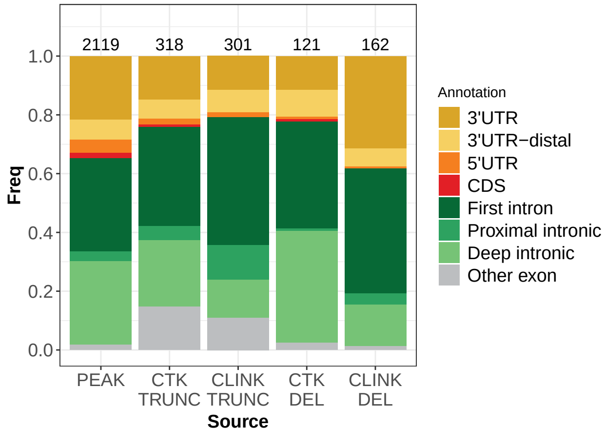
HNRNPC iCLIP Genic Annotation Proportions
