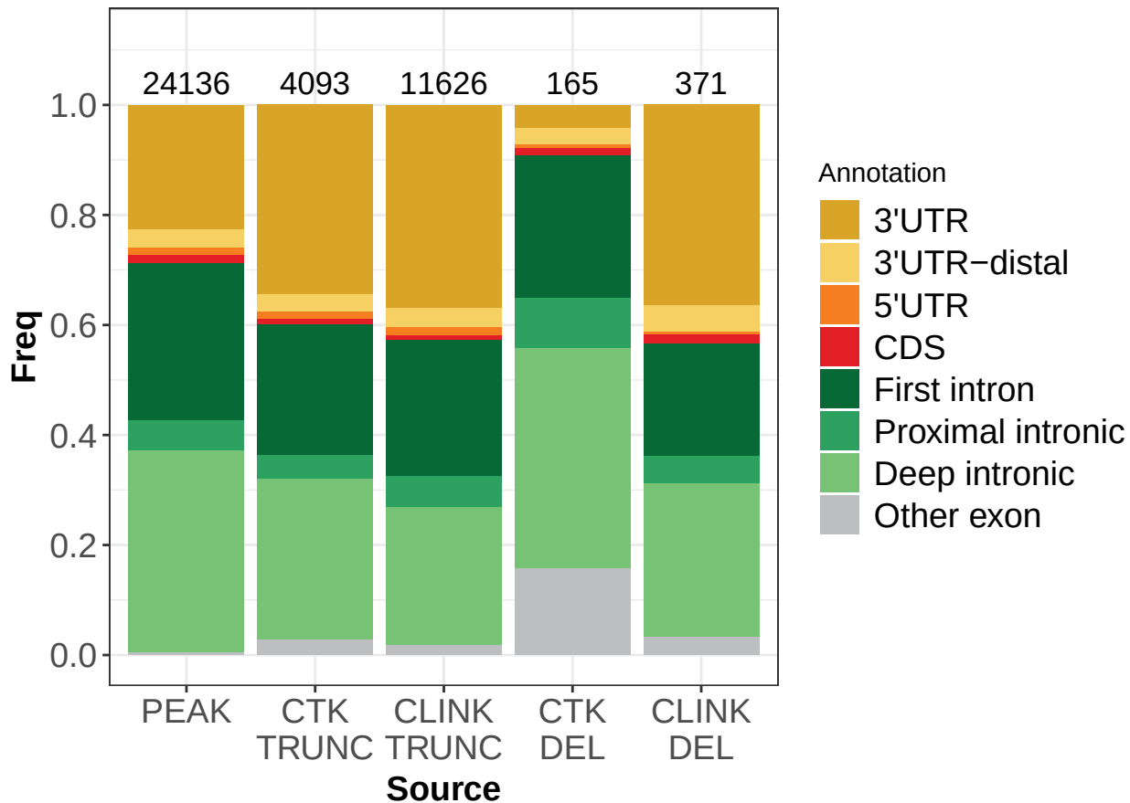
HuR CoCLIP Input Genic Annotation Proportions
