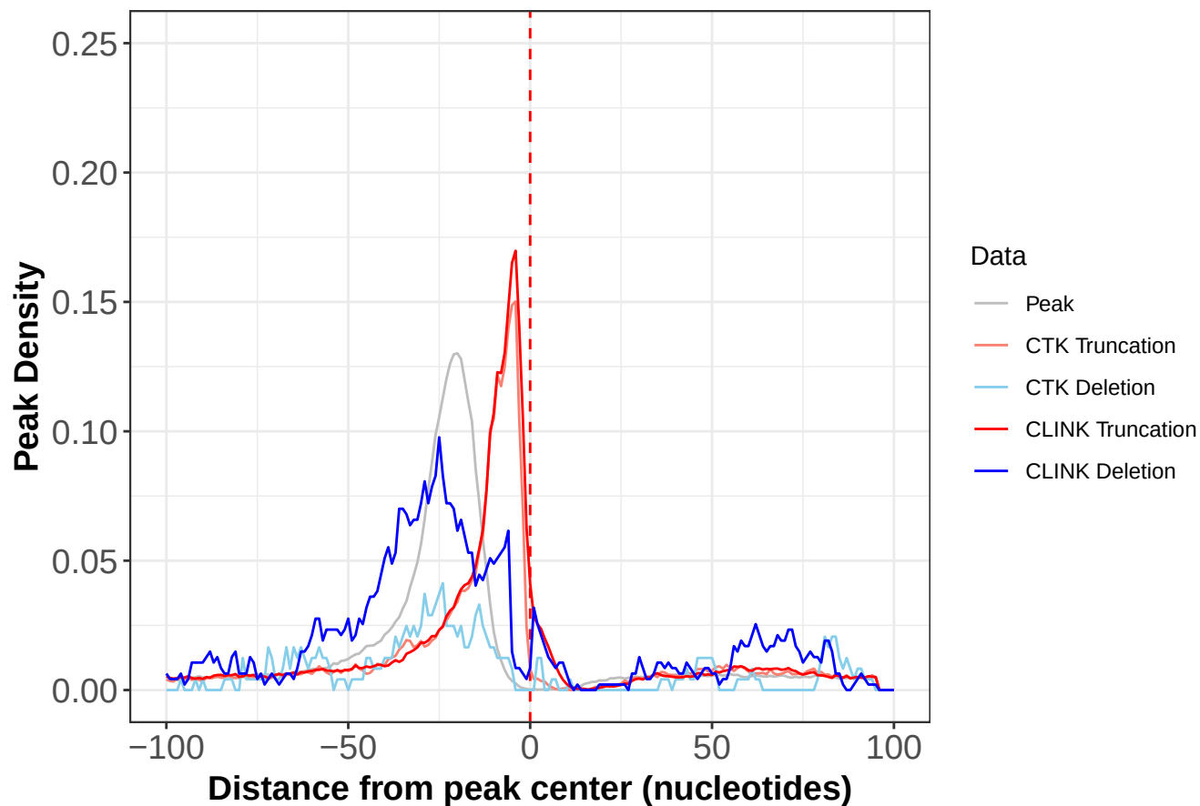
Motif Density around Peaks for HuR CoCLIP Input
