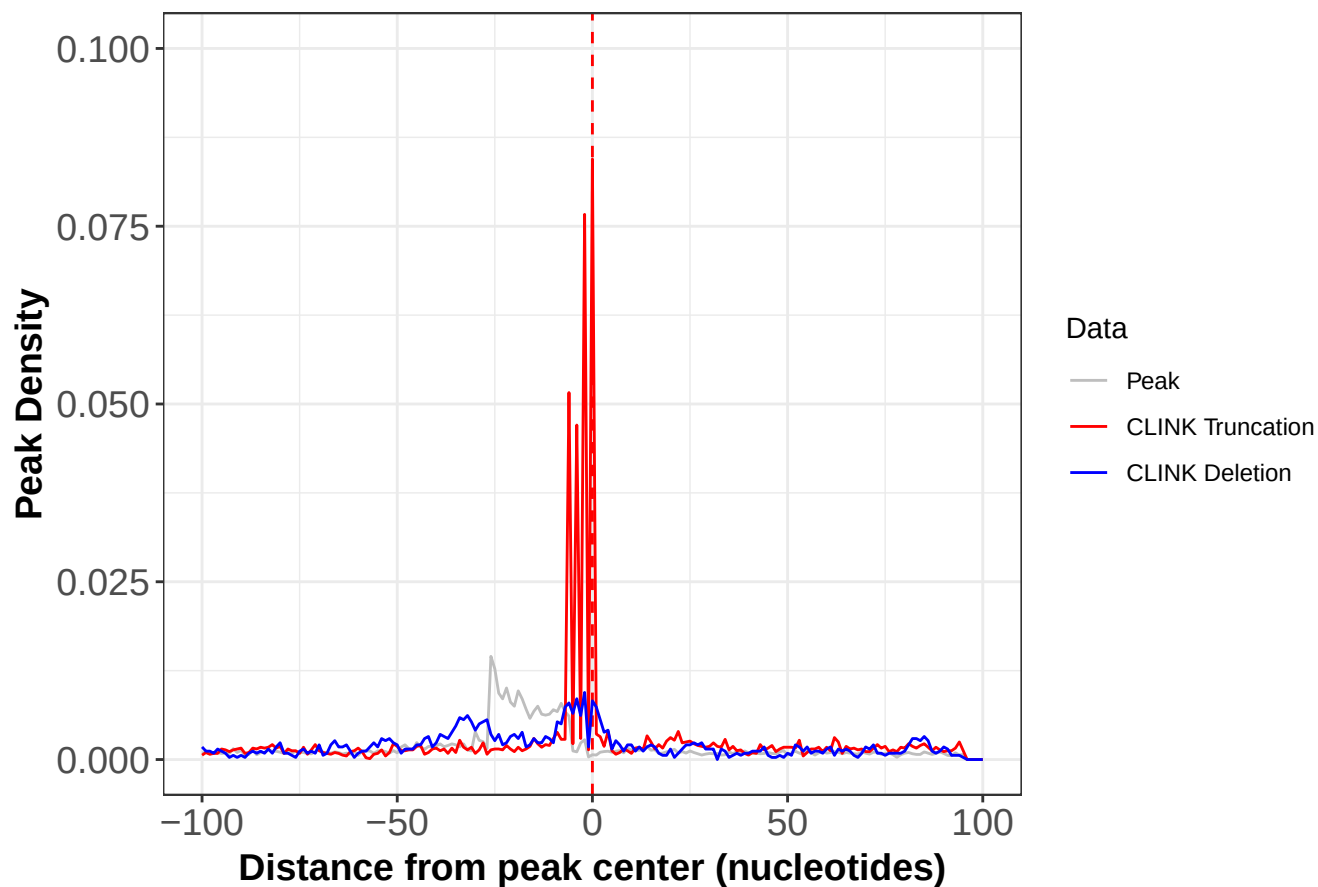
Motif Density around Peaks for RBFOX2 eCLIP HepG2
