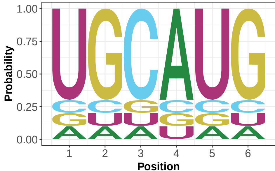
RBFOX2 eCLIP HepG2 PEAK motif
