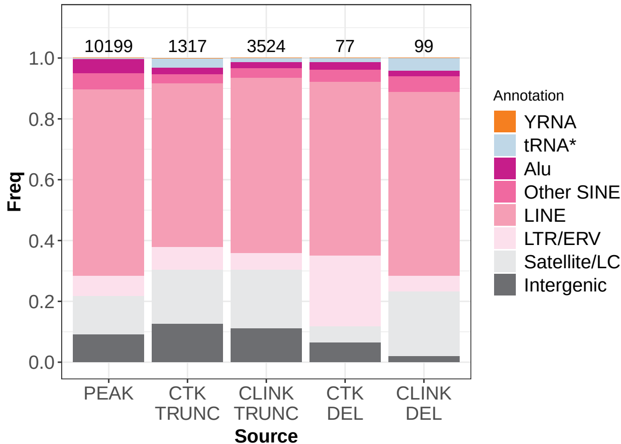
HuR CoCLIP Input Non-Genic Annotation Proportions
