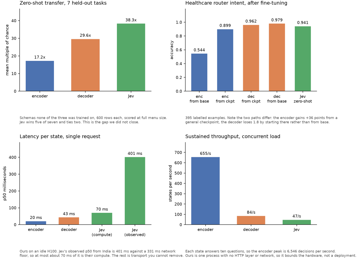
Figure 3: The two backbones and the commercial reference on the four questions a deployment actually asks. The reference system wins zero-shot transfer and we do not close that gap. Given a few hundred labels the ordering reverses, and on latency and sustained throughput it is not close. No single number summarises this, which is why we do not report one.
