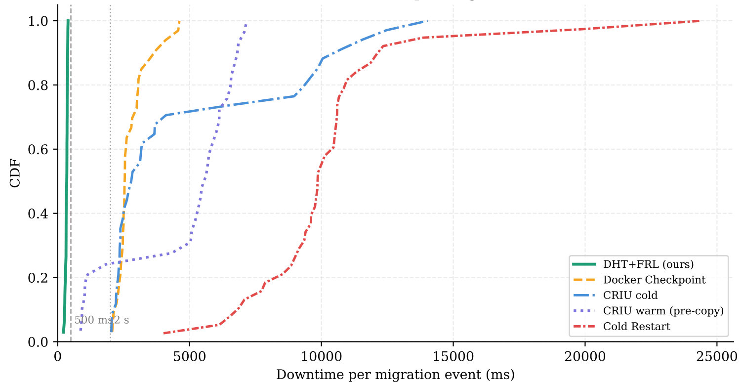
CDF of Robot Downtime per Migration Event
