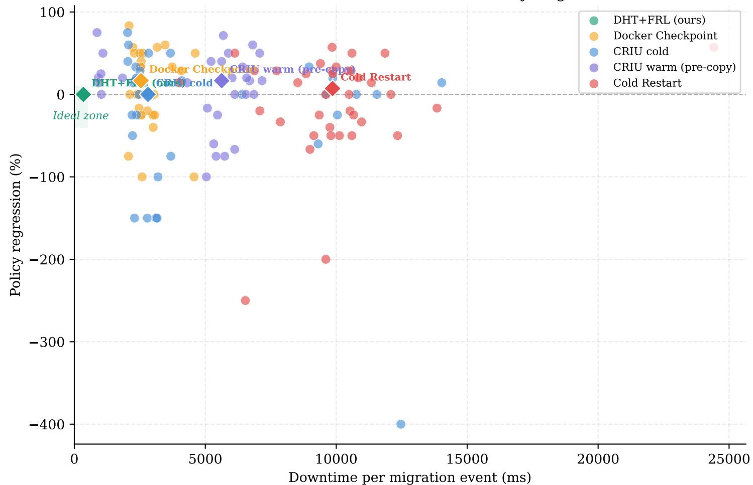
Per-Event Trade-off: Downtime vs. Policy Regression
