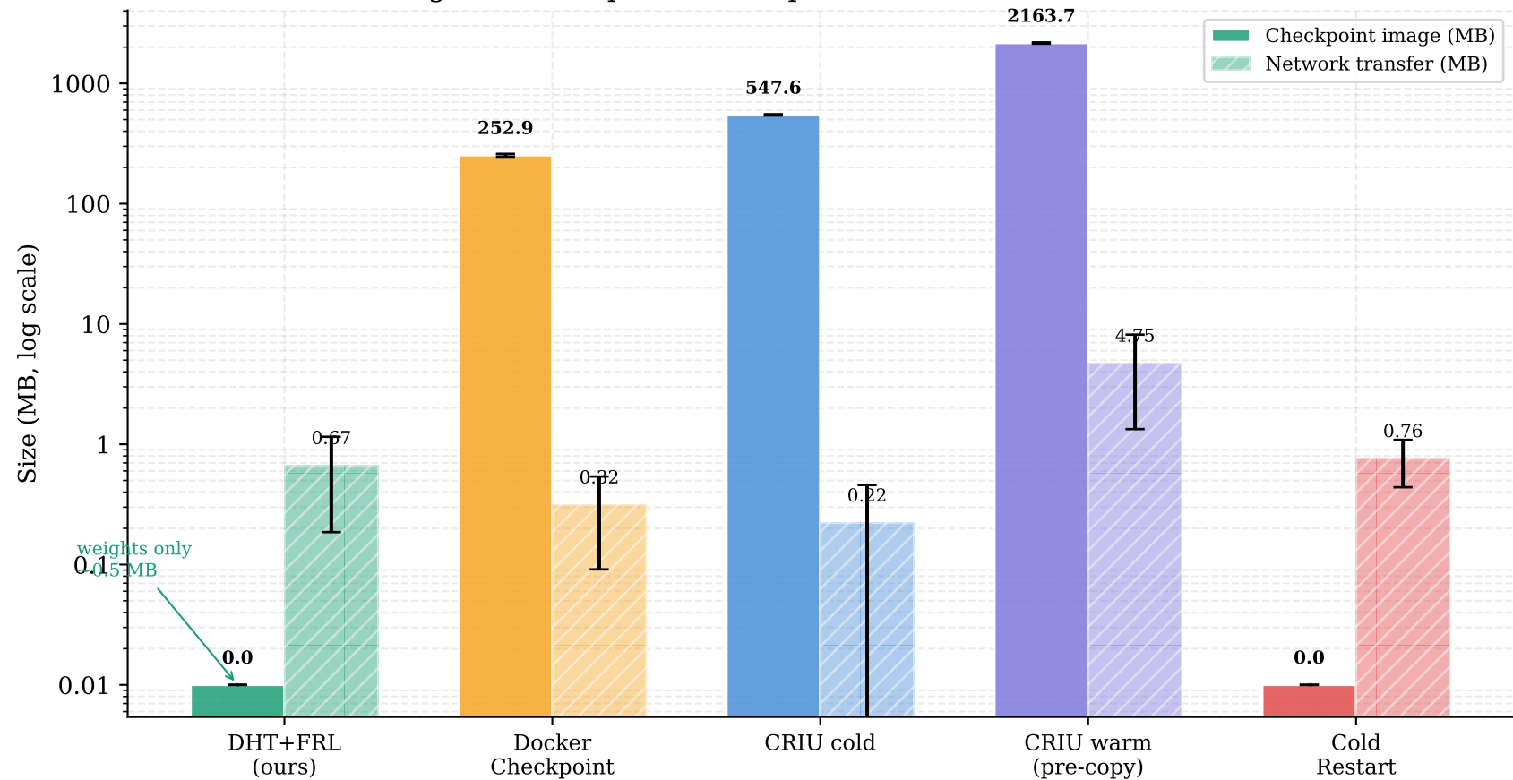
Migration Footprint: Checkpoint Size vs. Network Transfer
