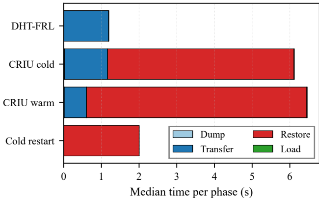
Where migration time goes: per-phase breakdown
