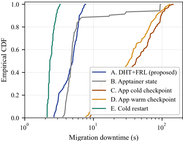
CDF of migration downtime
