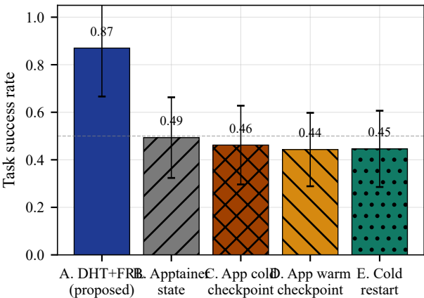
Task success rate per condition (mean \pm std)
