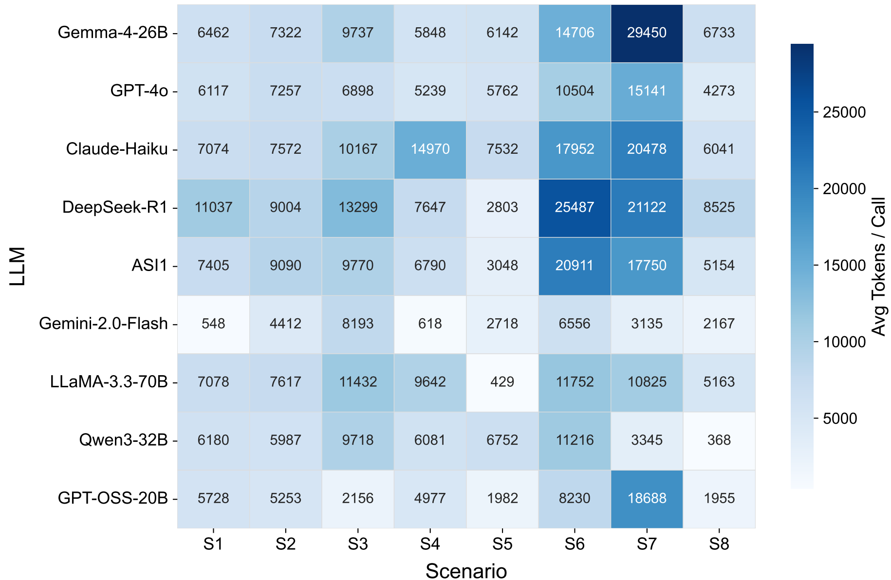
(a) Baseline
