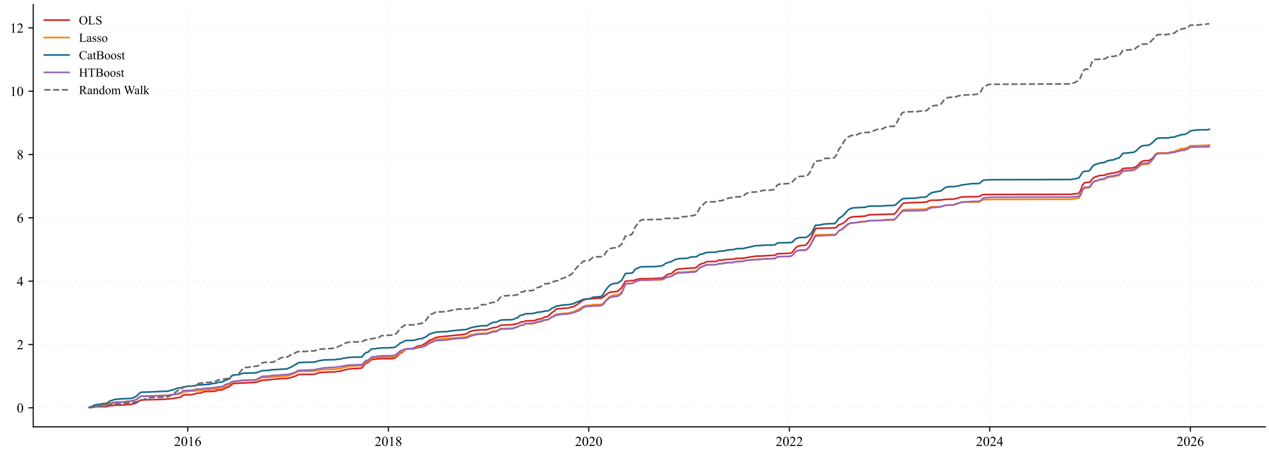
Purged k-fold — Cumulative Squared Error (1m, 543 shared dates)
