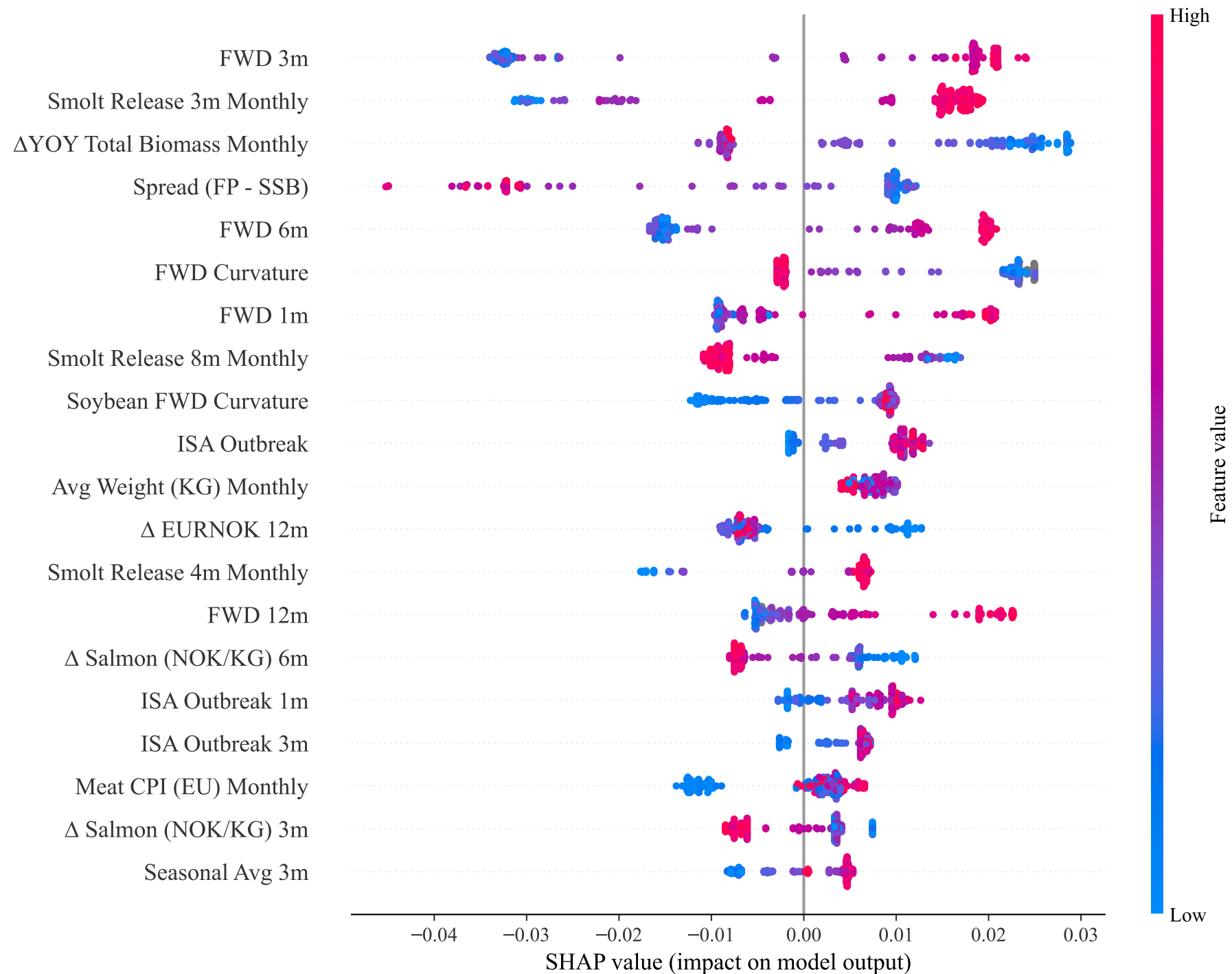
SHAP Beeswarm — CatBoost [MAE] | Y 3m \Delta Salmon (NOK/KG) Holdout 2022–2025 | Top 20 features | depth=2
