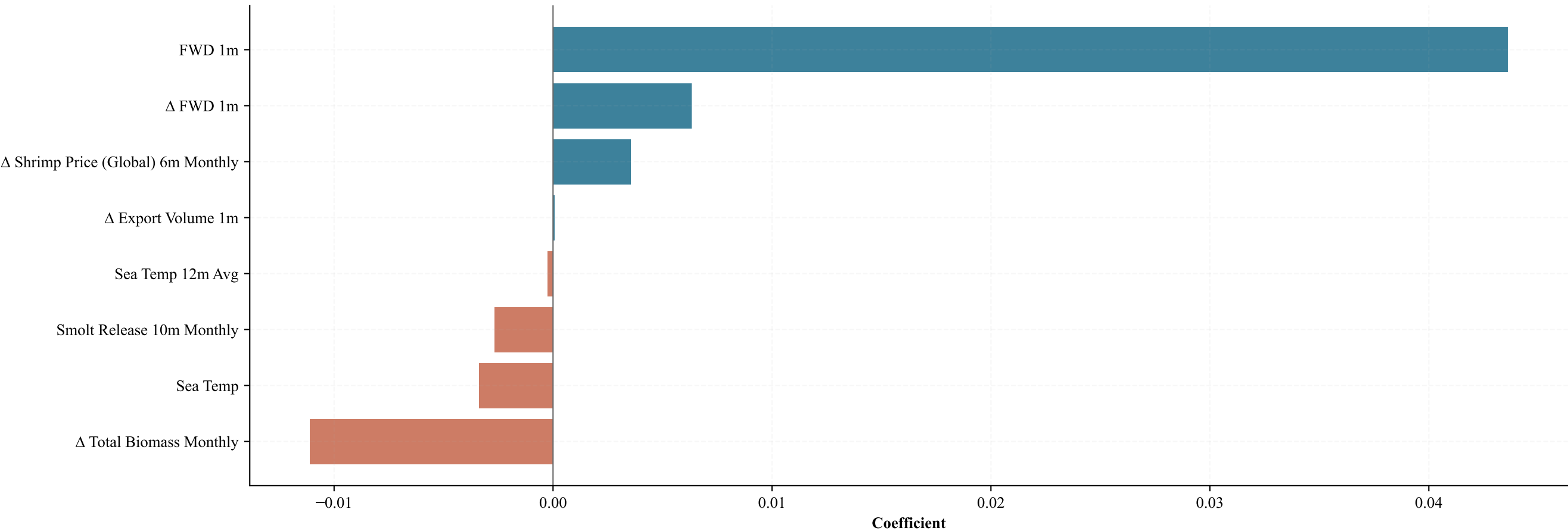
Non-zero Lasso Coefficients (8 selected, \alpha =0.00739)
