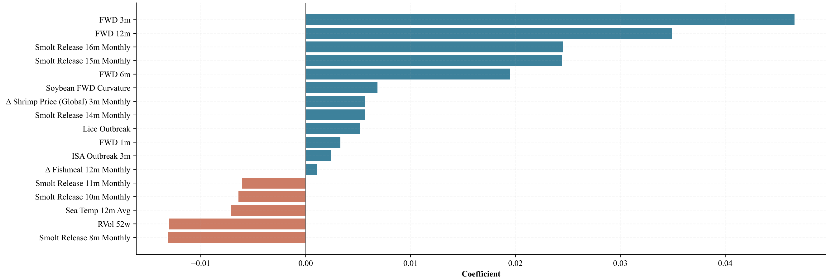
Non-zero Lasso Coefficients (17 selected, \alpha =0.01485)
