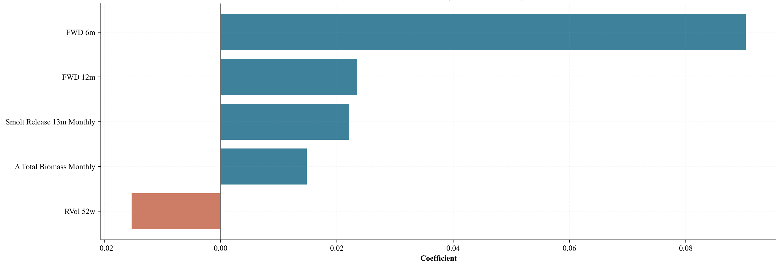
Non-zero Lasso Coefficients (5 selected, \alpha =0.03765)
