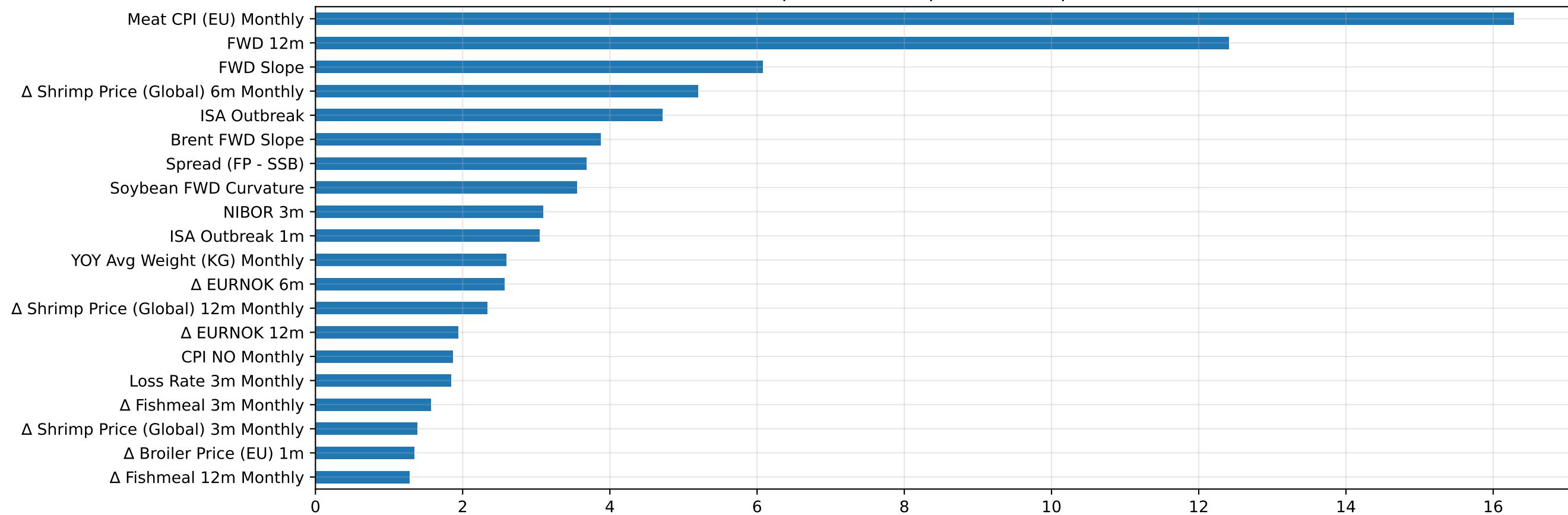
Top 20 feature importances (depth=5)
