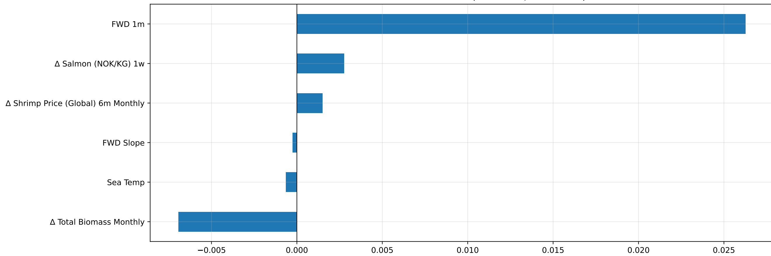
Non-zero Lasso coefficients (6 selected, \alpha=0.00521 )
