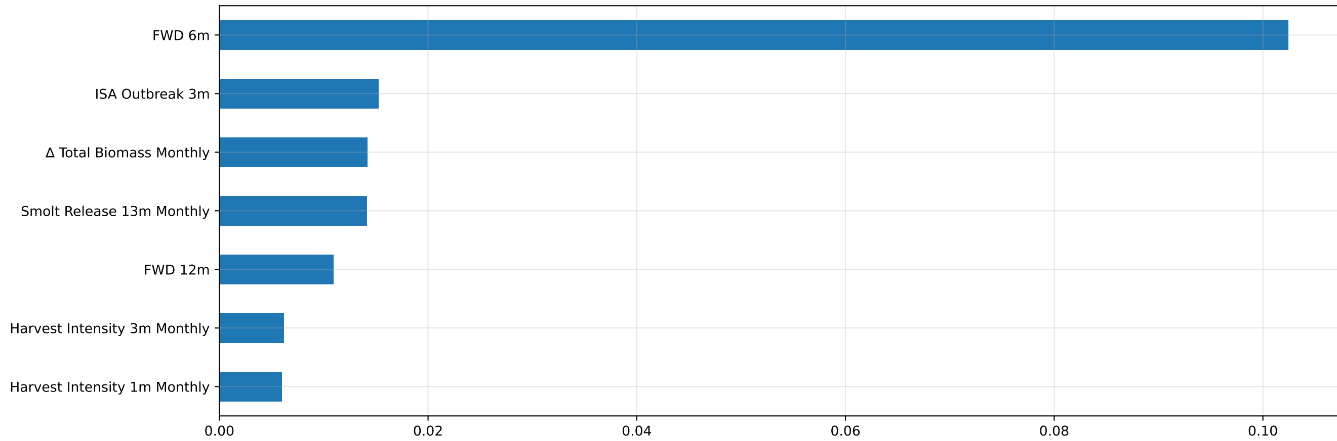
Non-zero Lasso coefficients (7 selected, \alpha=0.04229 )
