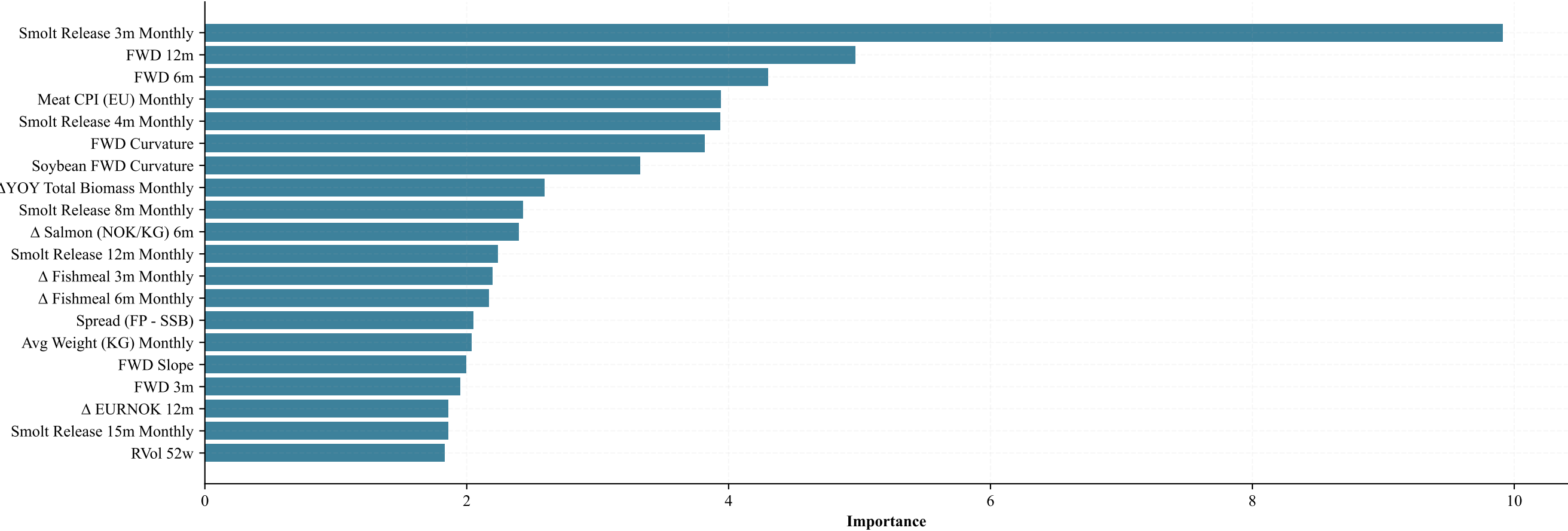
Top 20 Feature Importances (depth=5)
