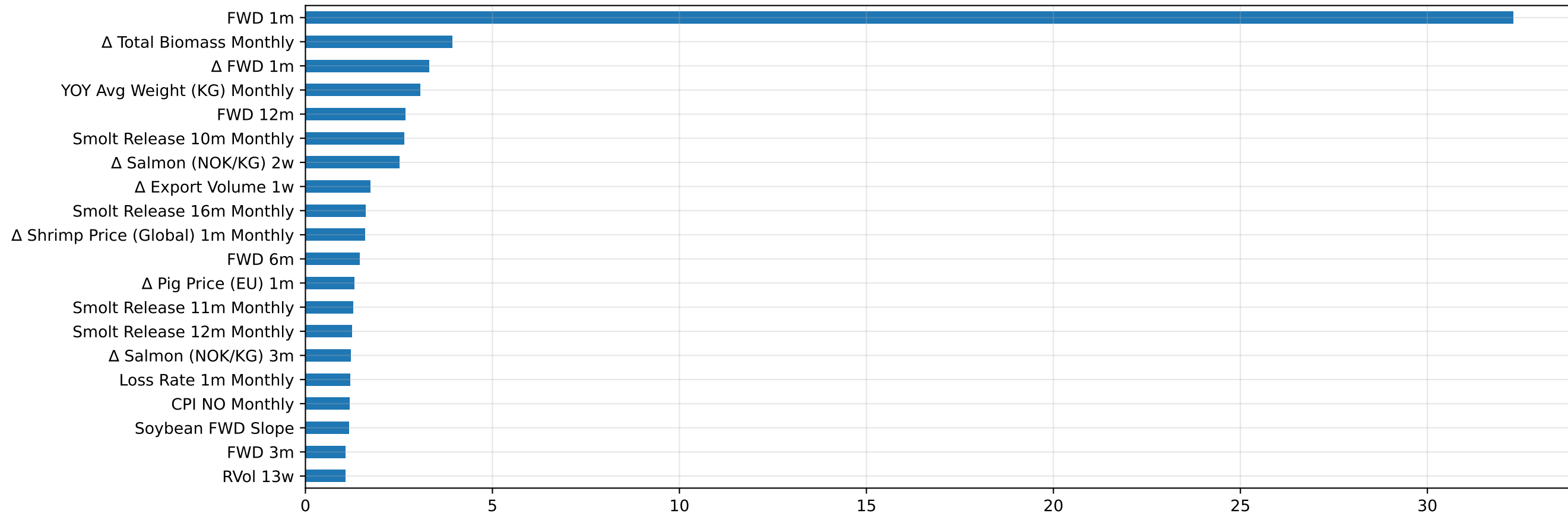
Top 20 feature importances (depth=4)
