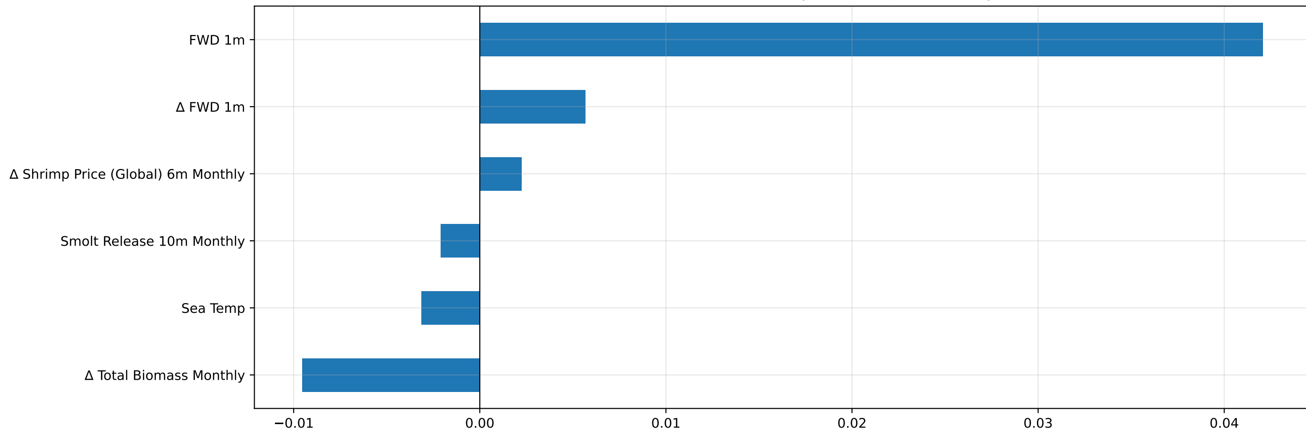
Non-zero Lasso coefficients (6 selected, \alpha =0.00830)
