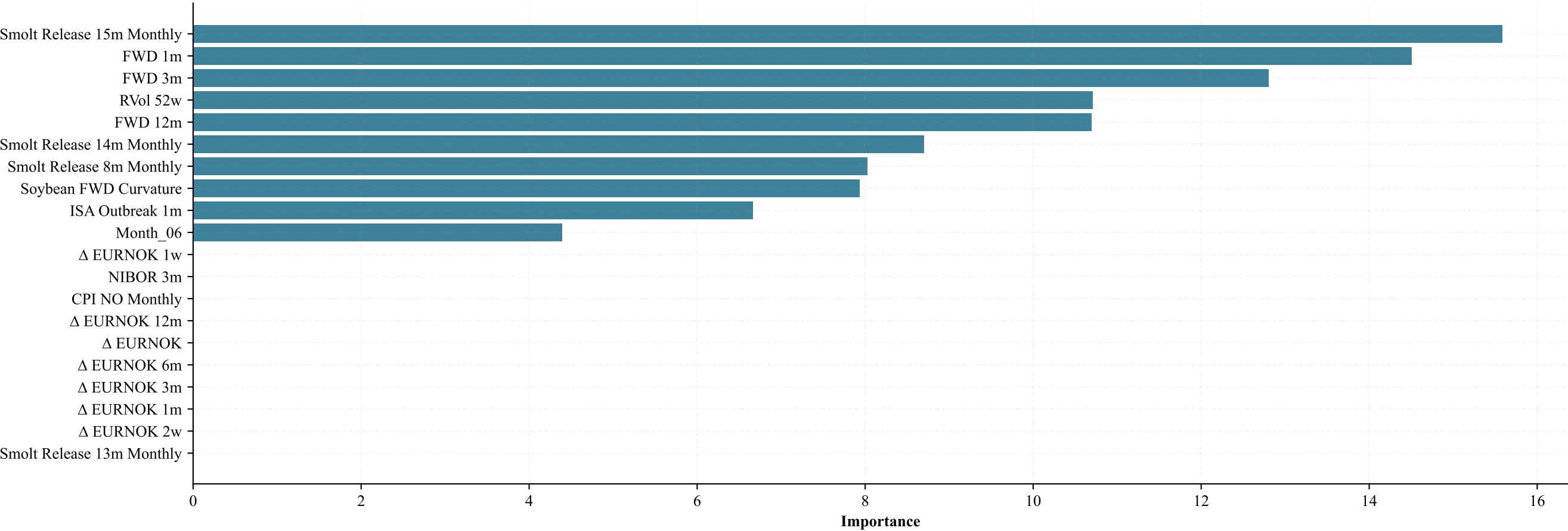
Top 20 Feature Importances — HTBrelevance (depth=2)
