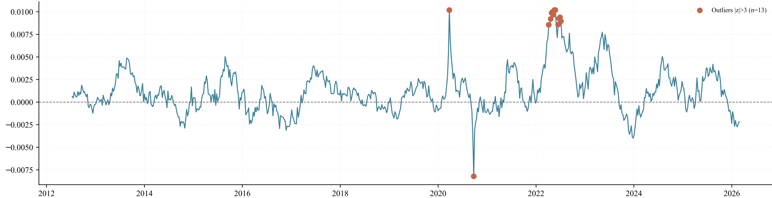
Time Series
