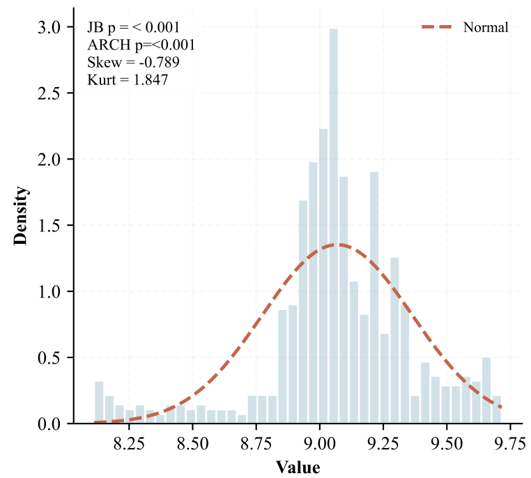
Distribution
