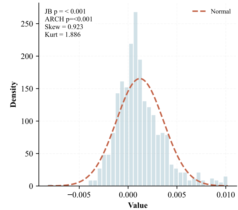
Distribution
