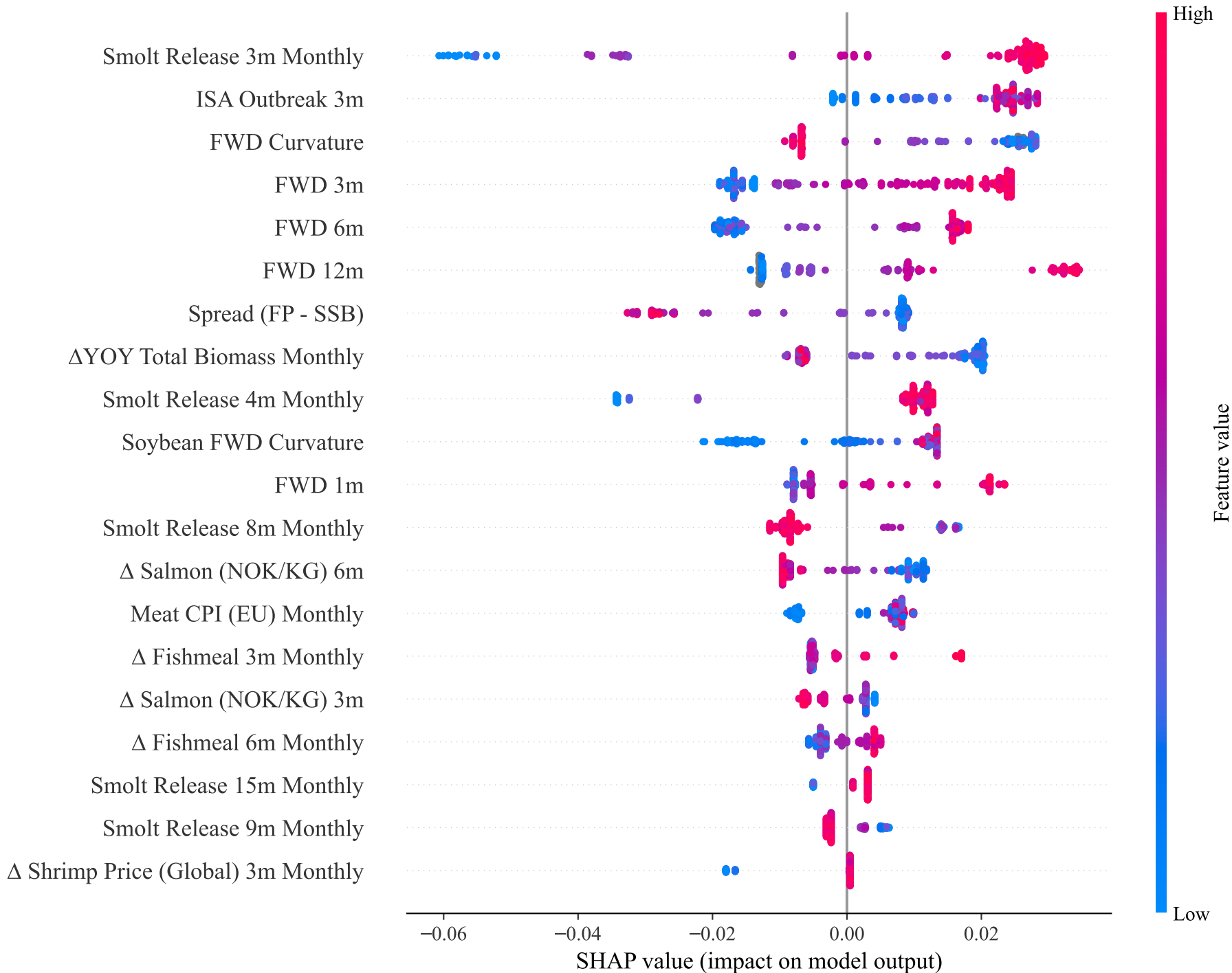
SHAP Beeswarm — CatBoost [RMSE] | Y 3m \Delta Salmon (NOK/KG) Holdout 2022–2025 | Top 20 features | depth=2
