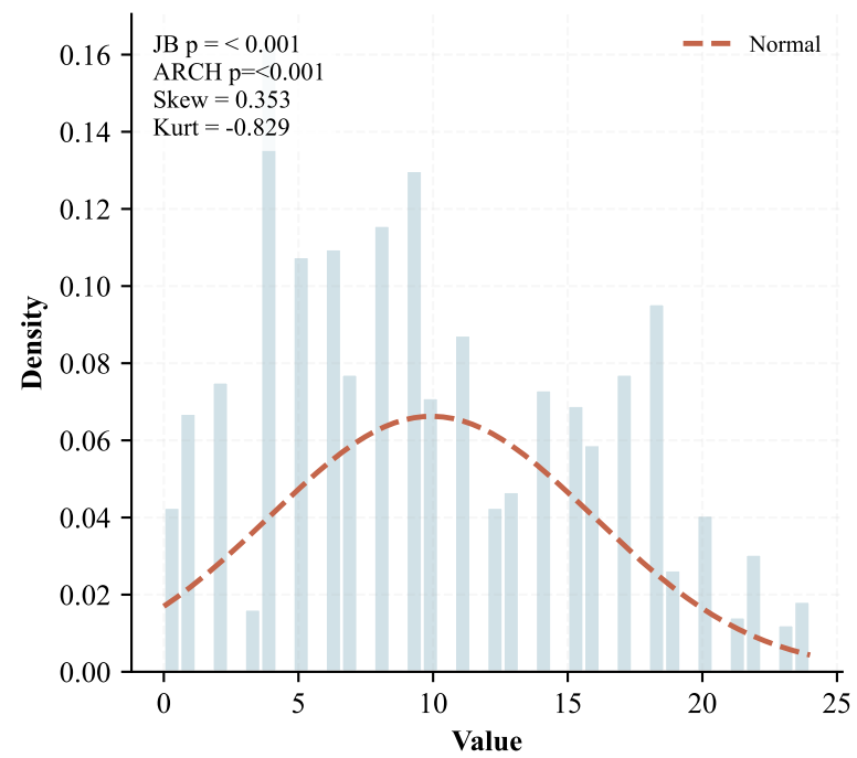
Distribution
