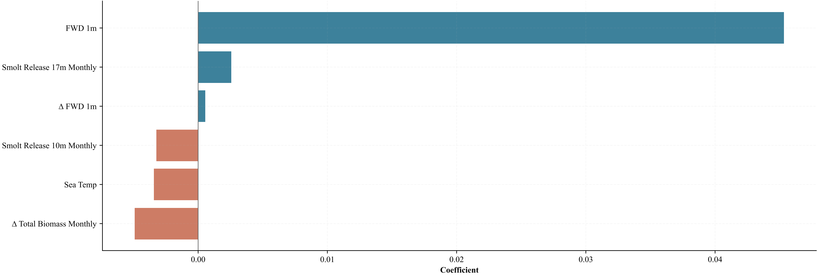
Non-zero Lasso Coefficients (6 selected, α=0.01177)
