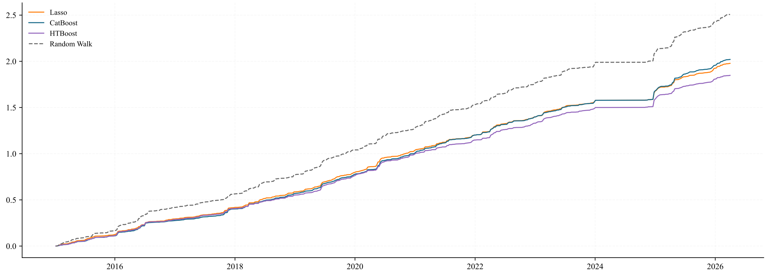
Purged k-fold — Cumulative Squared Error (0w, 546 shared dates)
