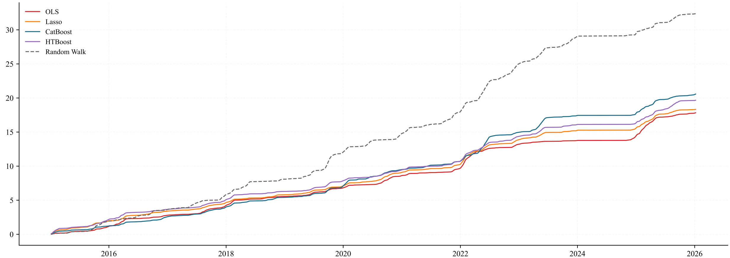
Purged k-fold — Cumulative Squared Error (3m, 534 shared dates)
