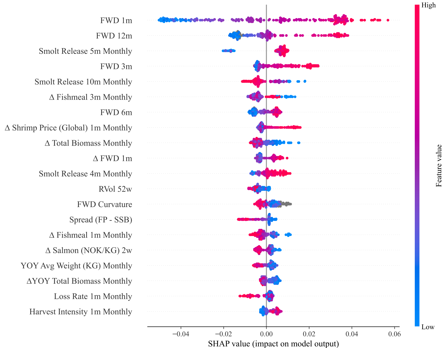
SHAP Beeswarm — CatBoost [RMSE] | Y 1m \Delta Salmon (NOK/KG) Holdout 2022–2025 | Top 20 features | depth=5
